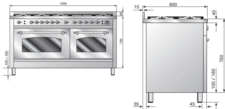
150cm Nostalgie 6 Burner + Simmer Plate Model PN150SMP Total Electrical Load (Kw) 7.4 Total Gas 'NG' Consumption (Mj/h) 73.8
