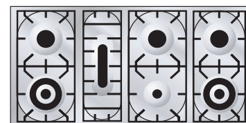
120cm Quadra 7 Burner Model PW1207MP Total Electrical Load (Kw) 5.7 Total Gas 'NG' Consumption (Mj/h) 76.3
