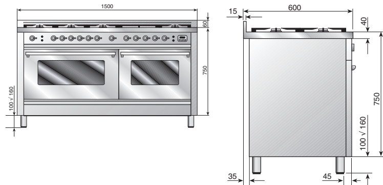
150cm Quadra 5 Burner + Tepanyaki & Simmer Plate Model PW150FSMP Total Electrical Load (Kw) 7.4 Total Gas 'NG' Consumption (Mj/h) 75
