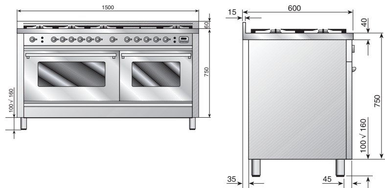
150cm Quadra 6 Burner + Simmer Plate Model PW150SMP Total Electrical Load (Kw) 7.4 Total Gas 'NG' Consumption (Mj/h) 73.8
