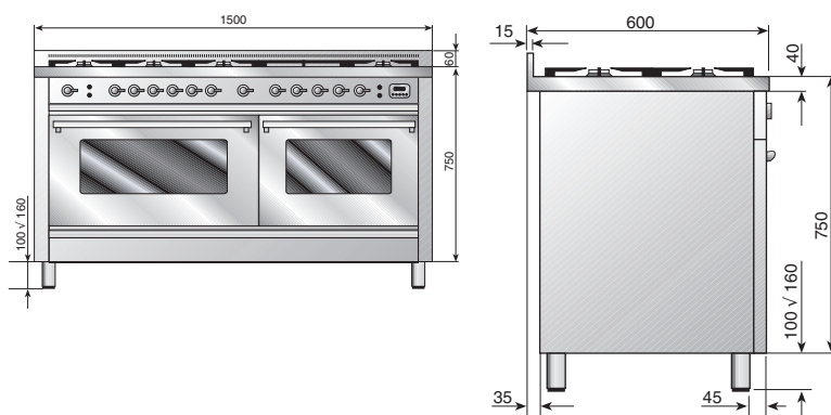
150cm Quadra 7 Burner + Ceran Model PW150VMP Total Electrical Load (Kw) 10 Total Gas 'NG' Consumption (Mj/h) 76.3
