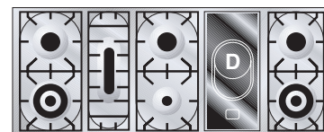
150cm Quadra 7 Burner + Ceran Model PW150VMP Total Electrical Load (Kw) 10 Total Gas 'NG' Consumption (Mj/h) 76.3
