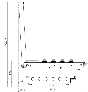
Supplied Hood ILBBQ124F: flat lid
